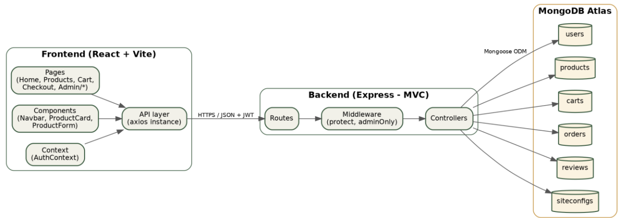
Figure 1: ShopEZ solution architecture — presentation, application, and data layers
